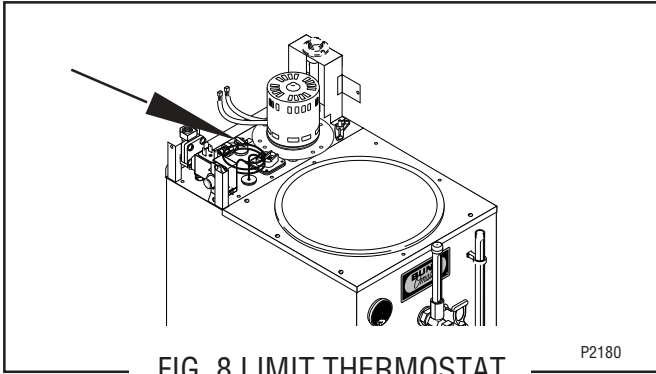
FIG. 8 LIMIT THERMOSTAT
