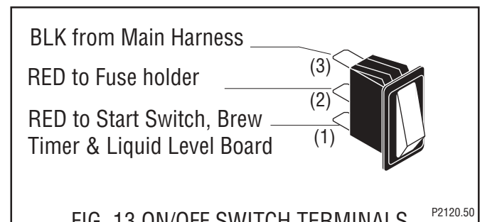
FIG. 13 ON/OFF SWITCH TERMINALS
