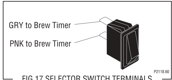
FIG.17 SELECTOR SWITCH TERMINALS
