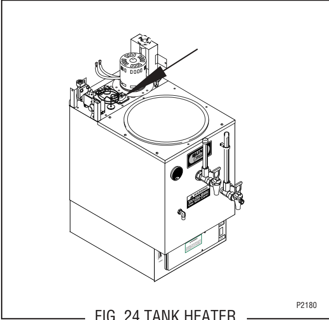
FIG. 24 TANK HEATER
